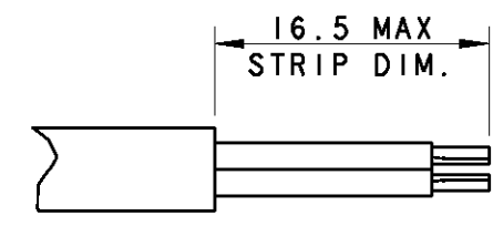
WIRE PREPARATION
